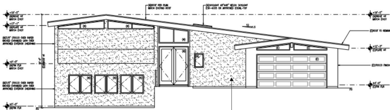
PROPOSED ELEVATION
