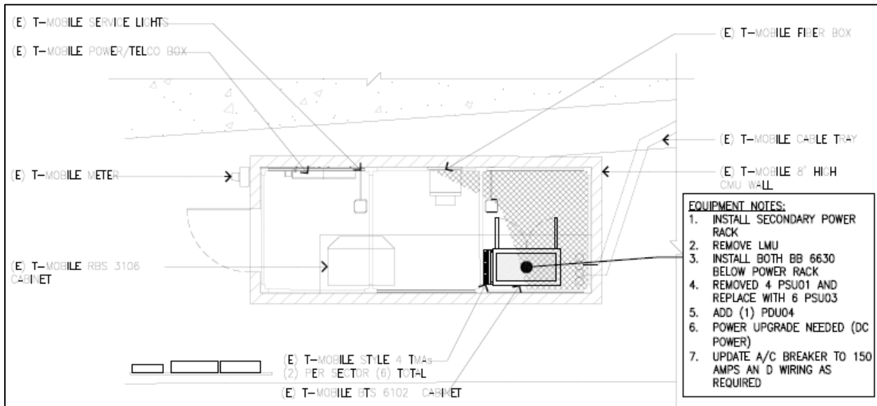
Figure 7: Proposed modifications in Verizon’s equipment room (Source: Plans, page A-2, panel 3).
