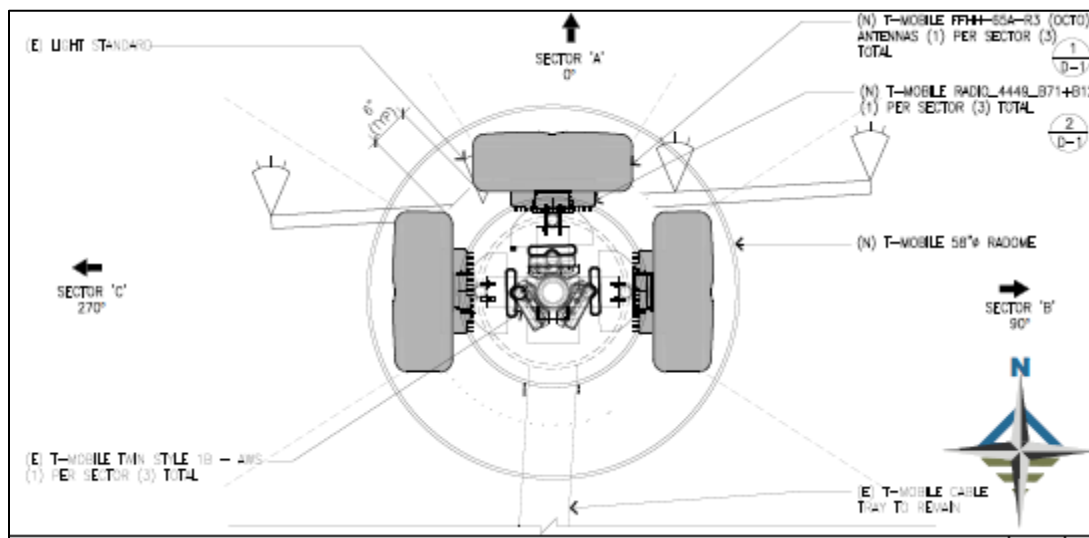
Figure 5: Proposed antenna layout plan (Source: Plans, page A-2, panel 3).
