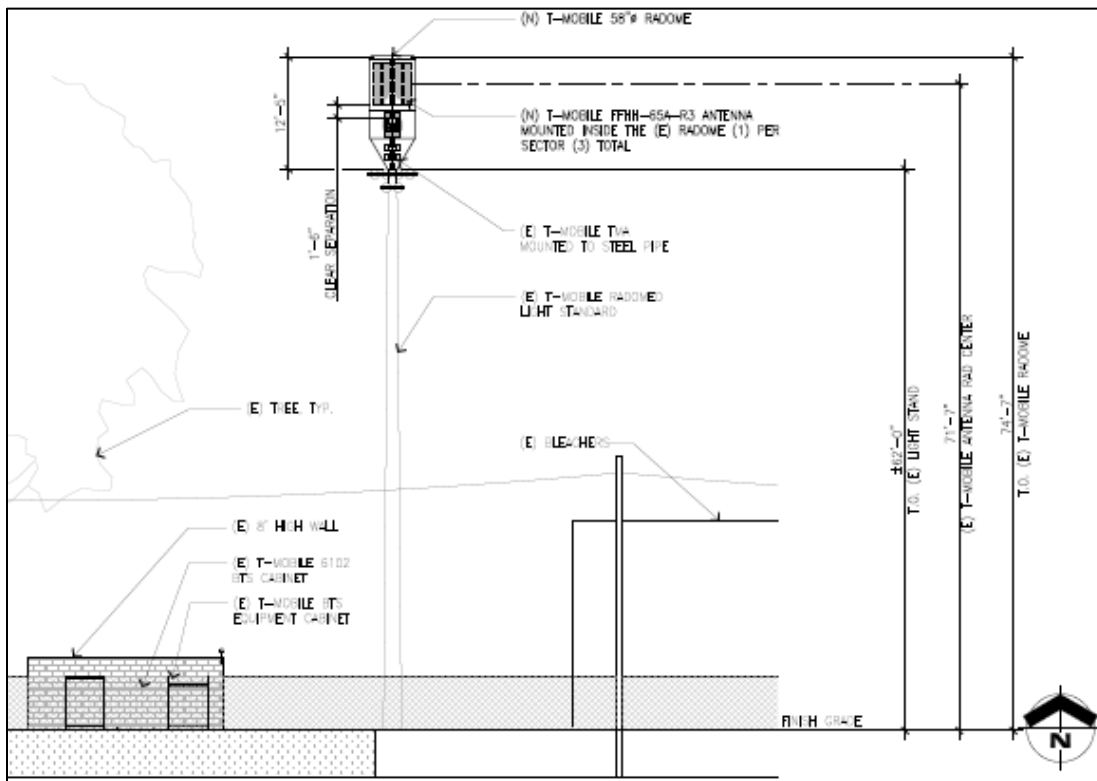
Figure 3: Elevation view of T-Mobile’s proposed wireless site. (Source: Plans, page A-3, panel 2).
