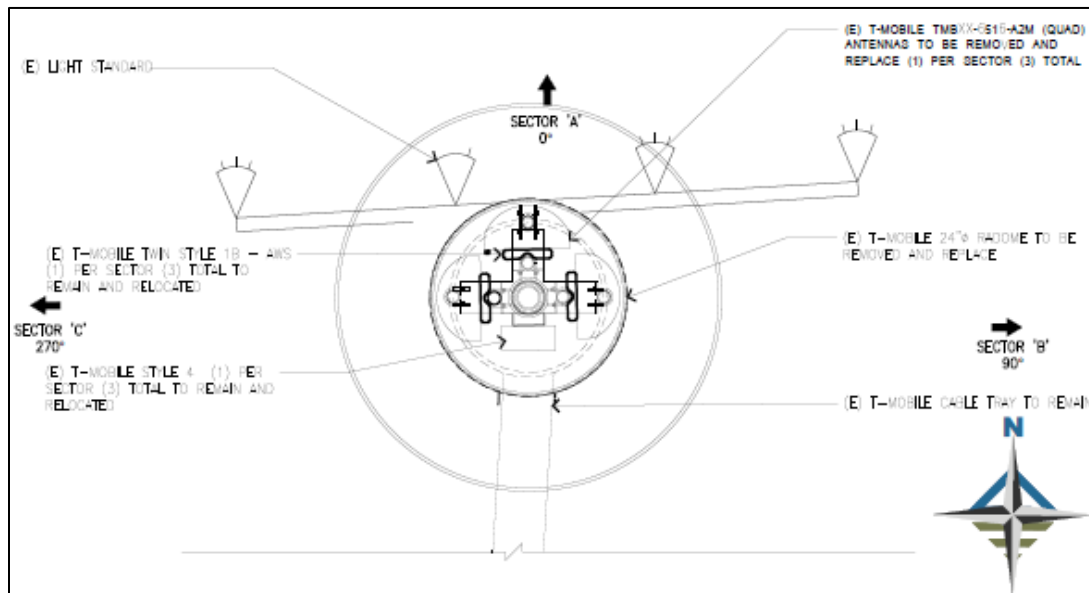
Figure 4: Existing antenna layout plan (Source: Plans, page A-2, panel 2).
